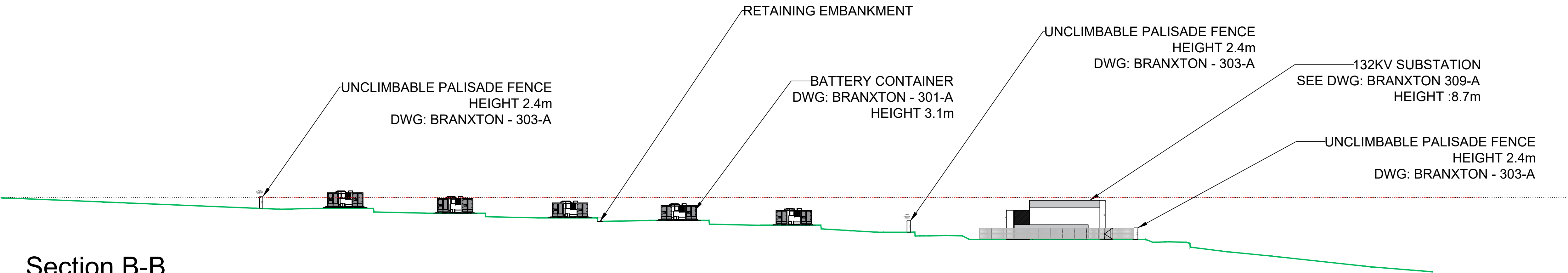
Section B-B
